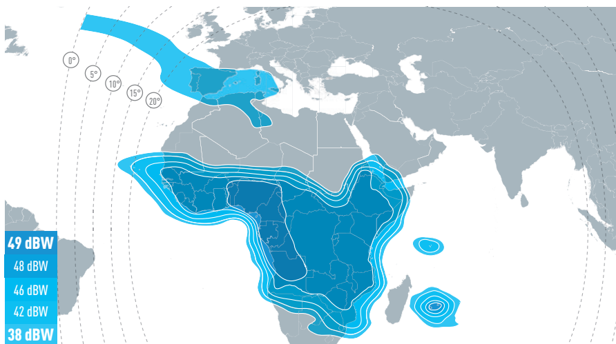
Ku-band Sub-Saharan Africa Downlink Coverage
