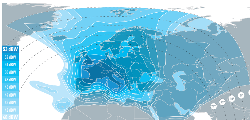
HOTBIRD 13C: Ku-band Widebeam Downlink Coverage
