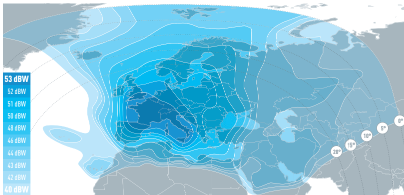
HOTBIRD 13B: Ku-band Widebeam Downlink Coverage
