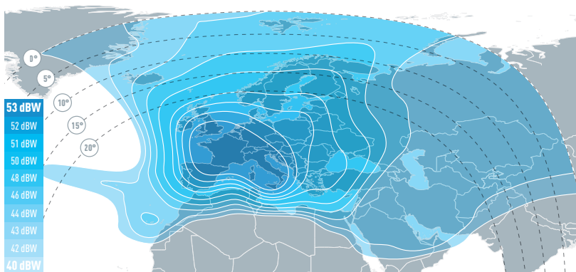
HOTBIRD 13E: Ku-band Widebeam Downlink Coverage
