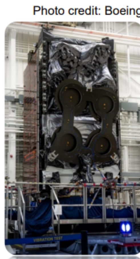
JCSAT-18 Photograph of construction
