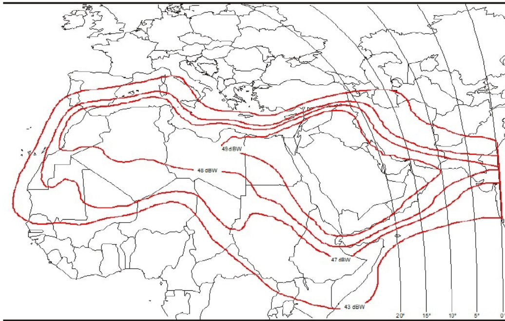
Nilesat 104 Ku-Band EIRP coverage
