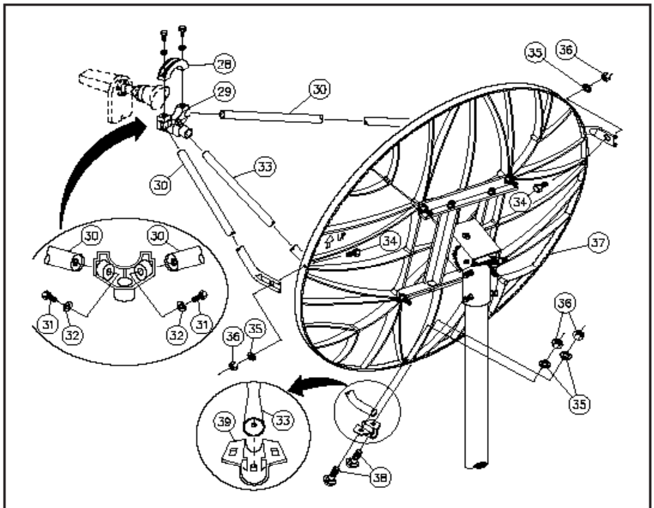
FIG. 3.2 - KU FEED SUPPORT LEGS
