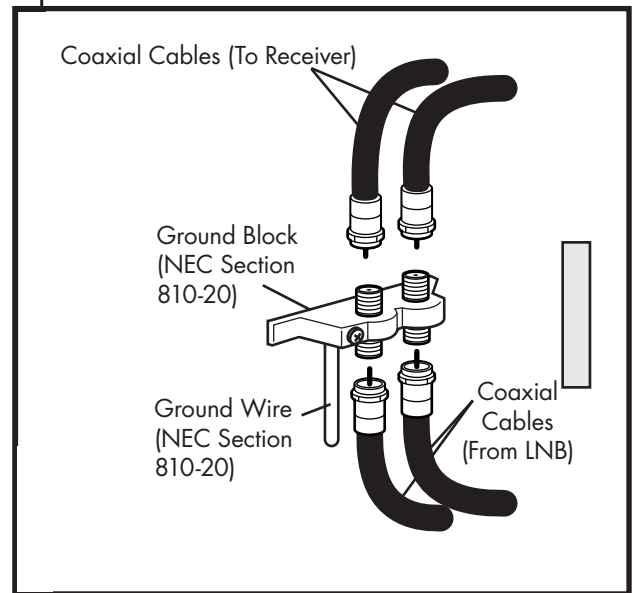
GROUNDING FEED CABLES
