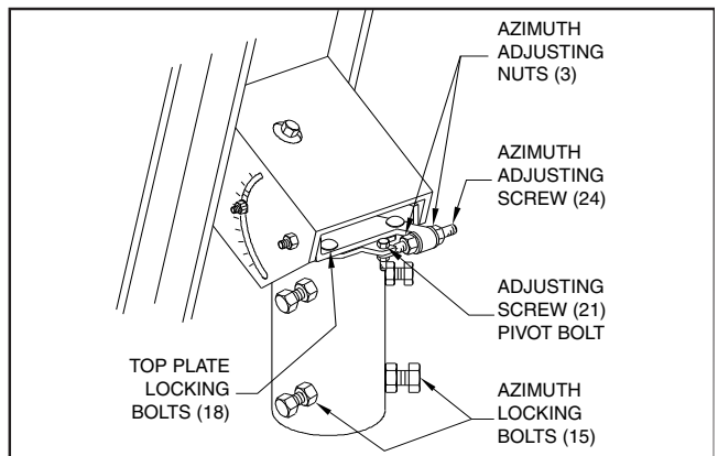
FIG. 2.3 - AZ/EL CAP MOUNT w/AZ FINE TUNE
