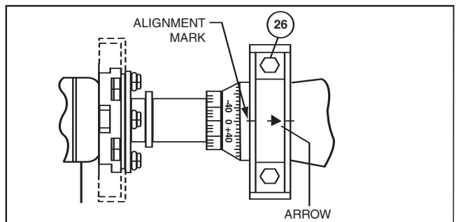
FIG. 2.2 - POLARIZATION OF FEED
