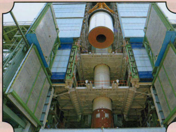
PS1 Segment Stacking
