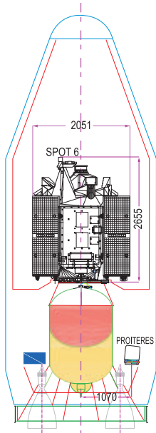
SPOT 6 and PROITERES in PSLV-C21 Envelope
