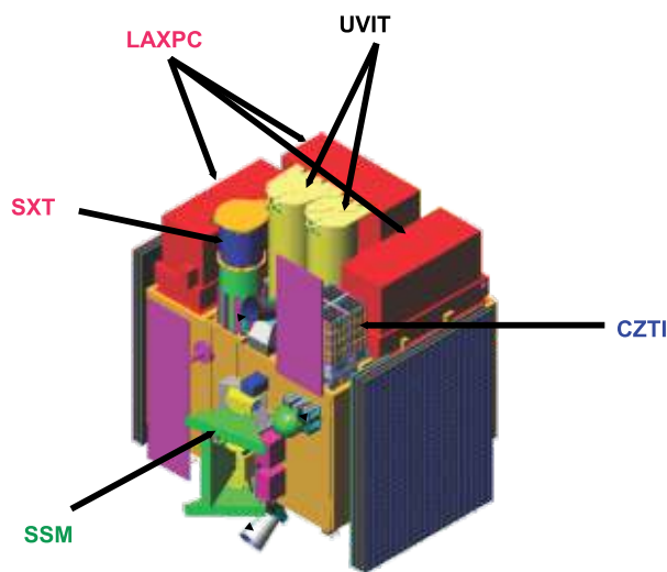
Astrosat Payload Locations
