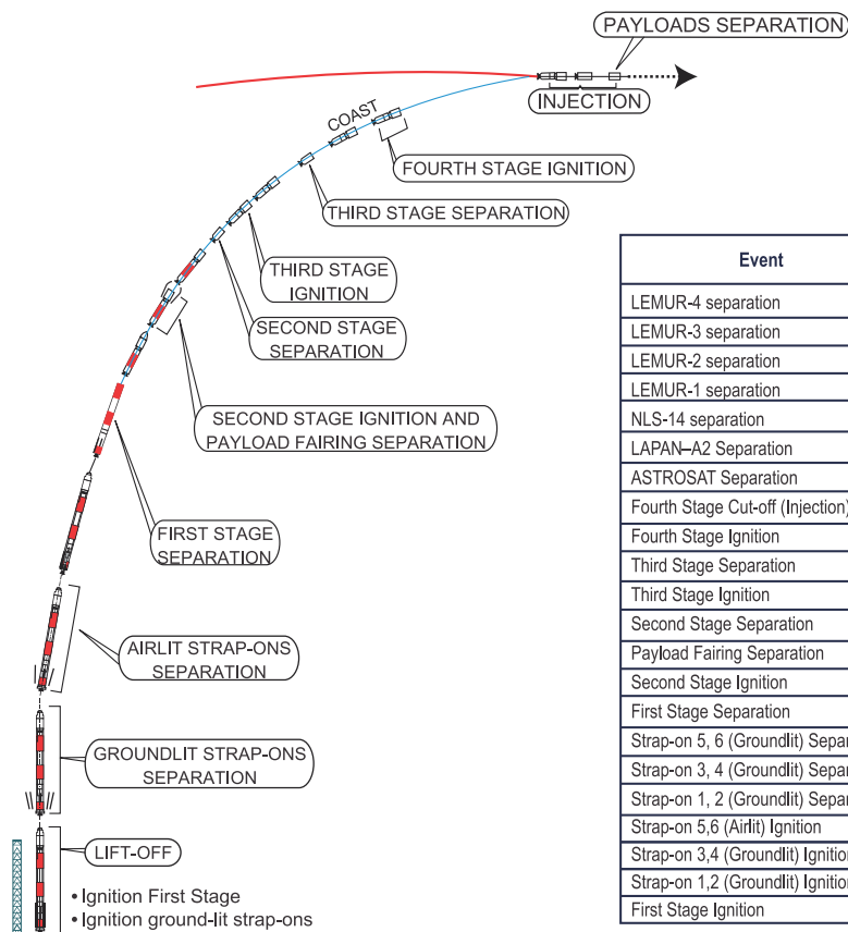
PSLV-C30 Typical Flight Profile
