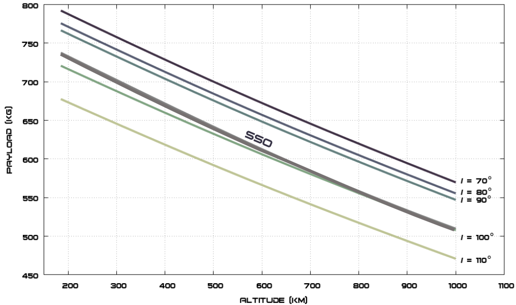
FIGURE 4 Alpha West Coast Performance Capability for Popular Inclinations
