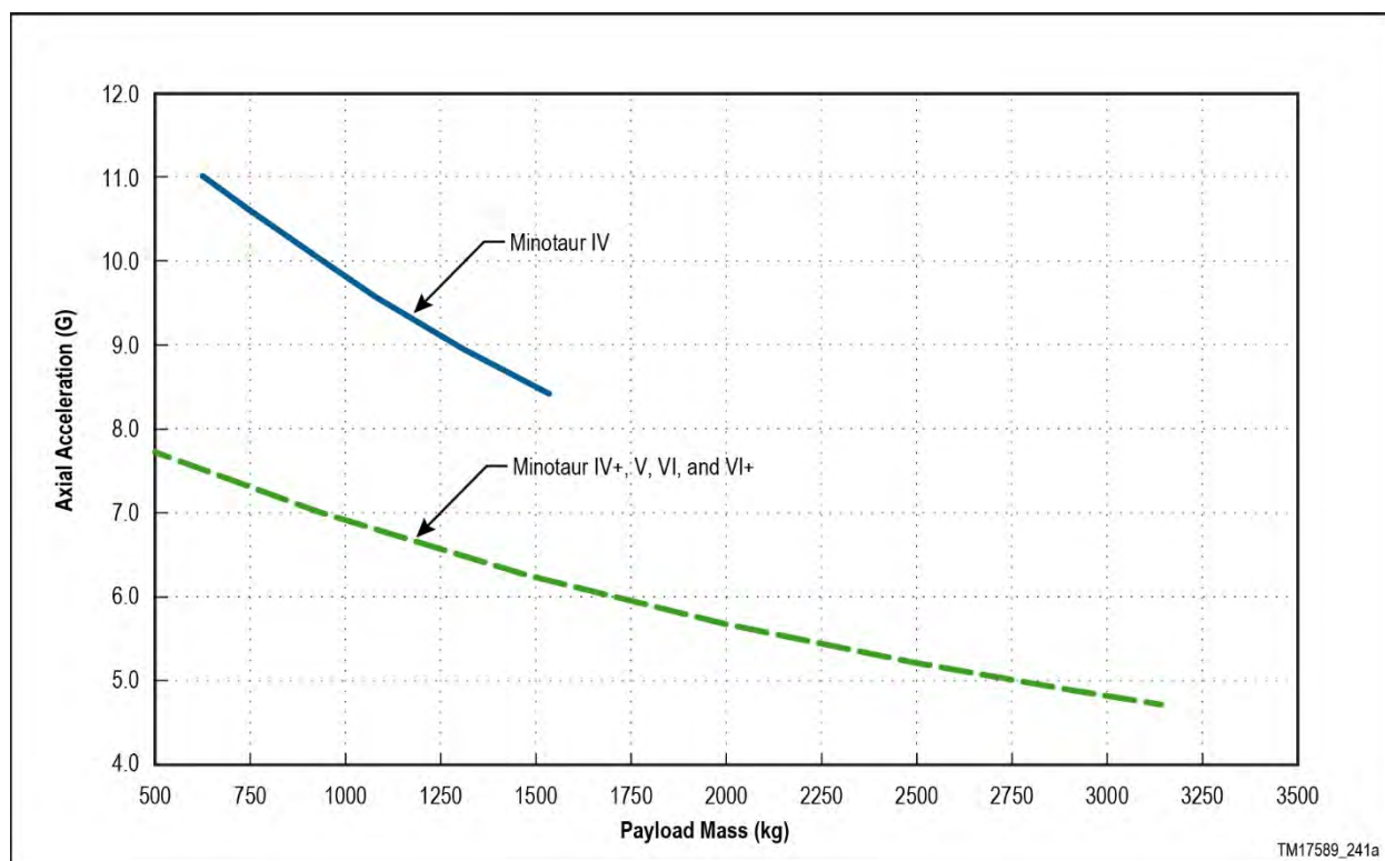
Figure 4.1.2-1. Minotaur IV Family Maximum Axial Acceleration as a Function of Payload Mass
