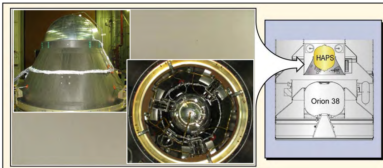
Figure 8.9-1. Hydrazine Auxiliary Propulsion System (HAPS) Used to Provide Insertion Accuracy
