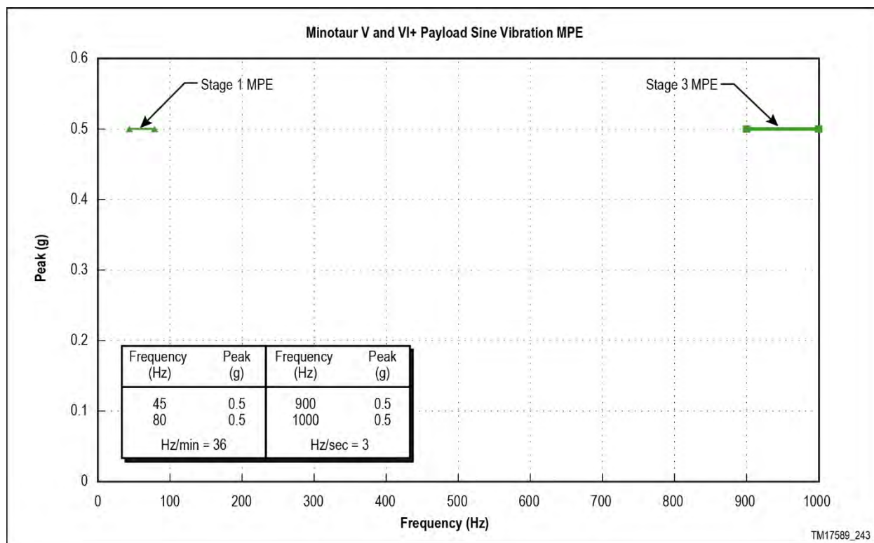
Figure 4.2.2-2. Minotaur V and VI+ Payload Sine Vibration MPE Levels
