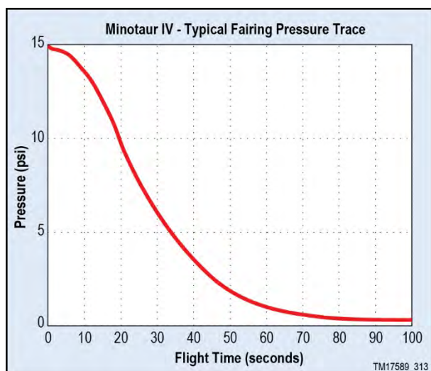
Figure 4.6.2-1. Typical Minotaur IV Fairing Pressure Profile
