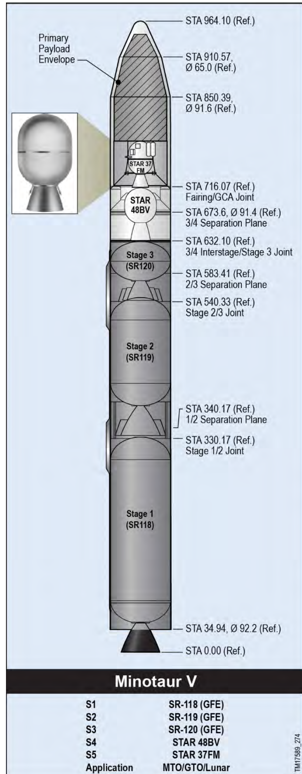
Figure 2.3.6.2-1. Minotaur V Vehicle Configuration
