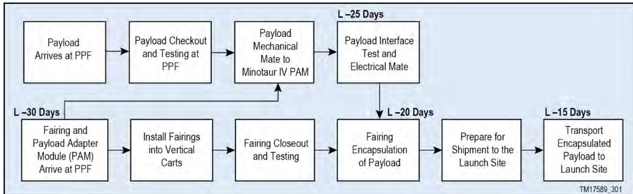
Figure 7.2-1. Payload Processing and LV Integration Flow at the PPF
