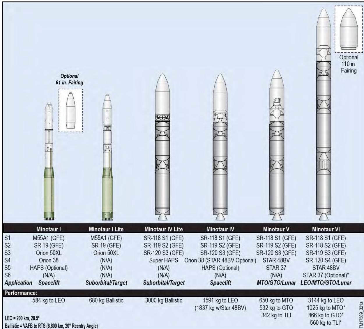
Figure 1.1-1. The Minotaur Family of Launch Vehicles
