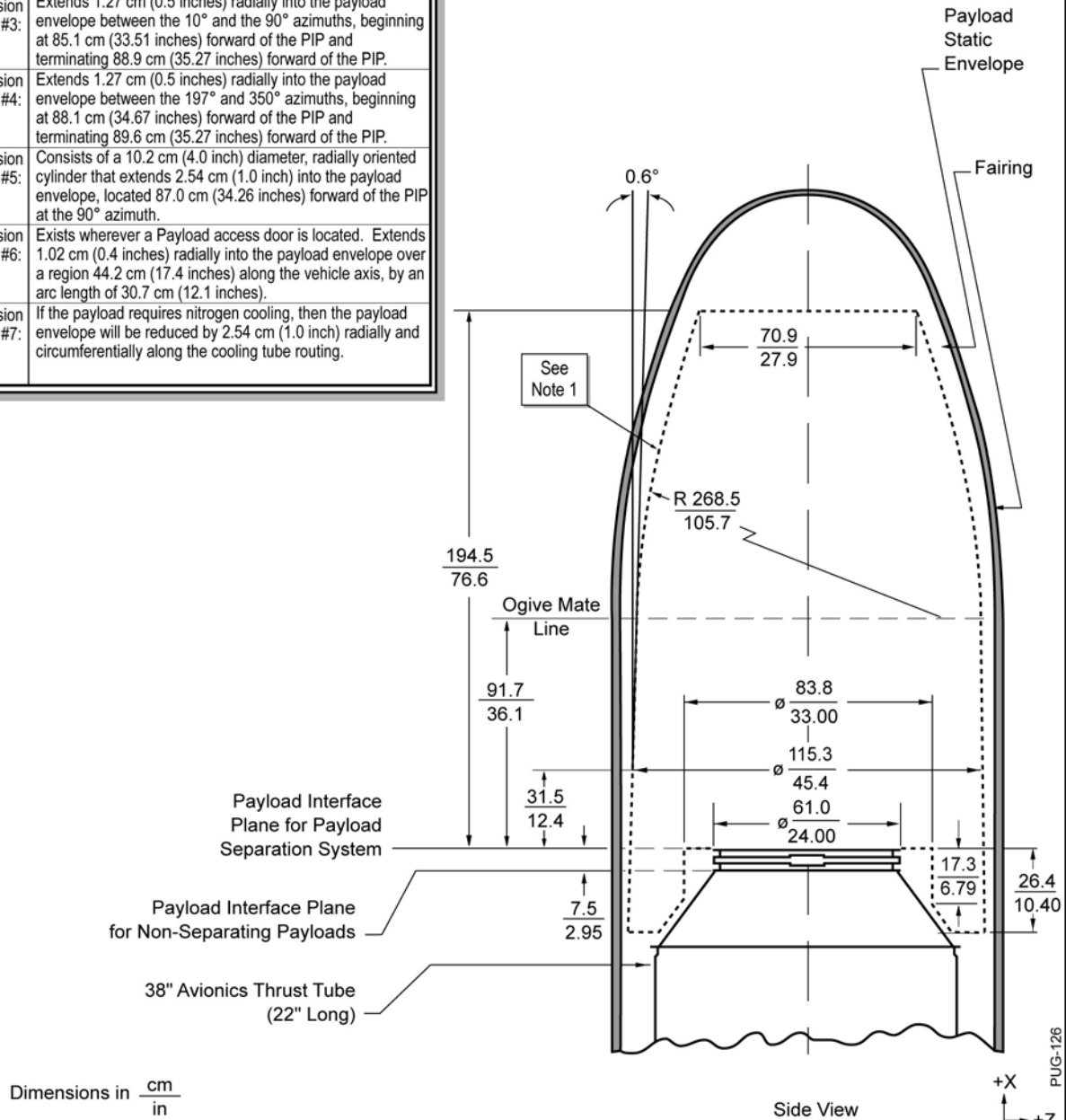
Figure 5-3. Payload Fairing Static Envelope with 59 cm (23 in.) Diameter Payload
