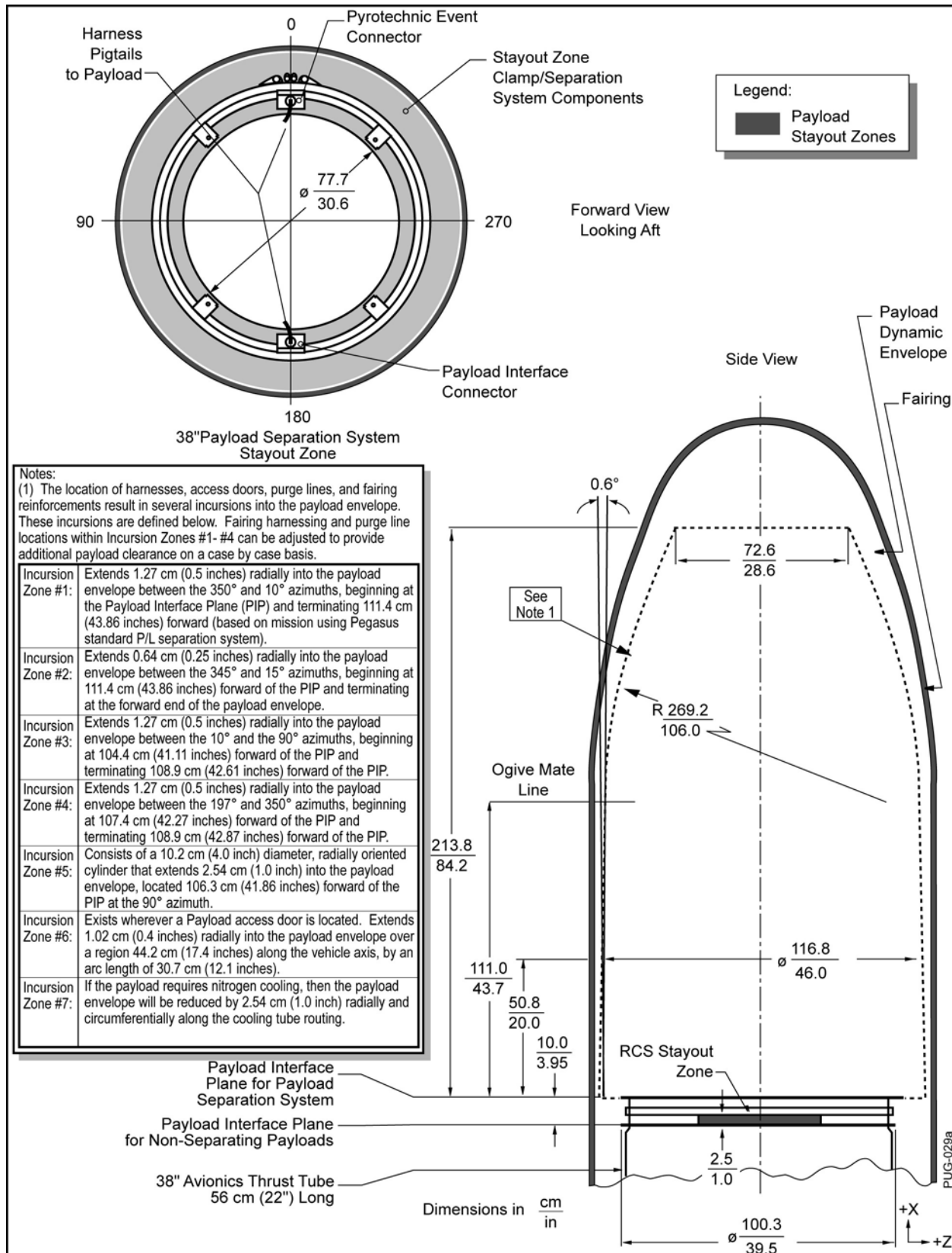
Figure 5-2. Payload Fairing Dynamic Envelope with 97 cm (38 in.) Diameter Payload
