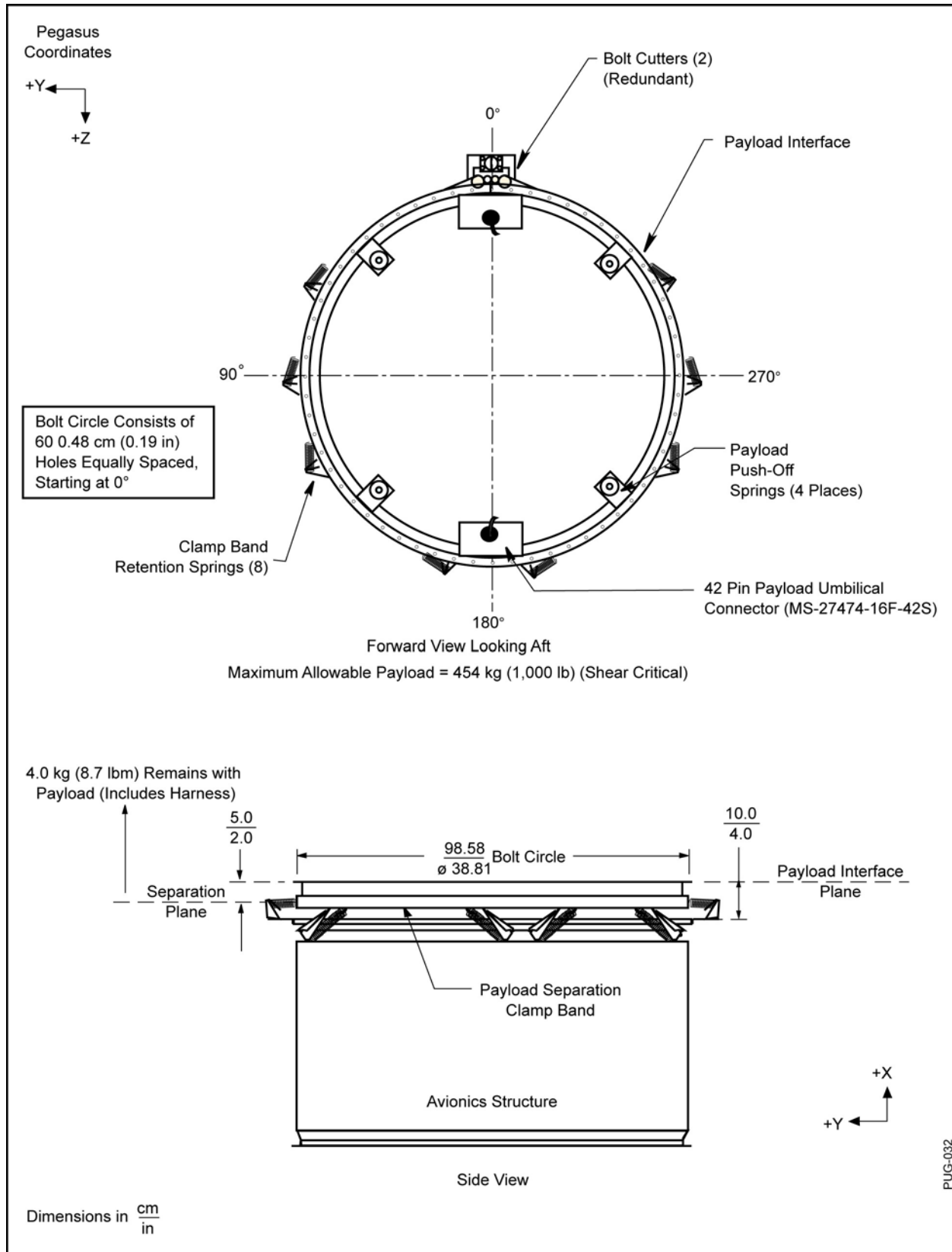
Figure 5-7. 97 cm (38 in.) Separable Payload Interface
