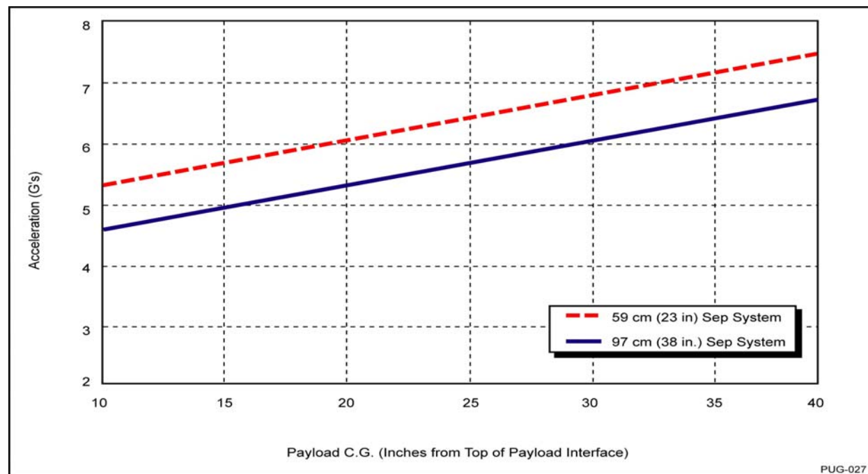
Figure 4-5. Pegasus Net CG Load Factor Predictions
