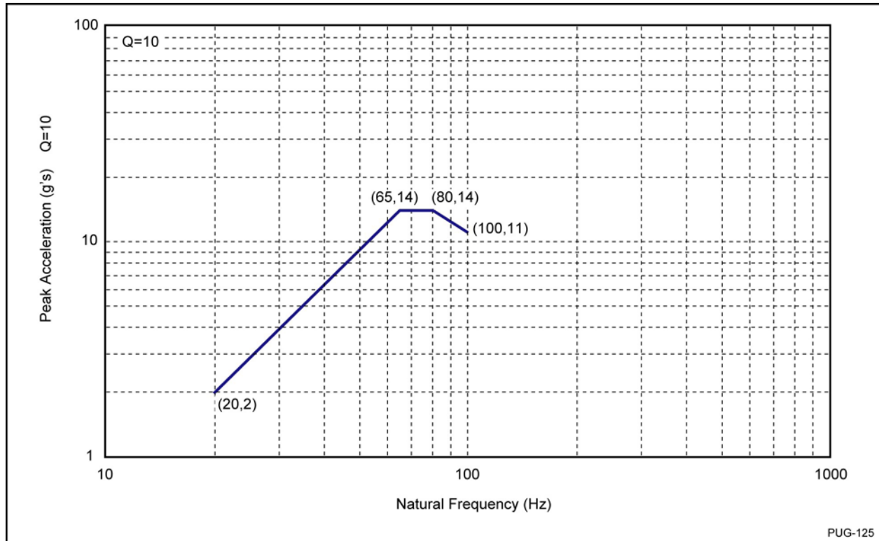
Figure 4-6. Motor Ignition Transient Shock Response Spectrum Specification
