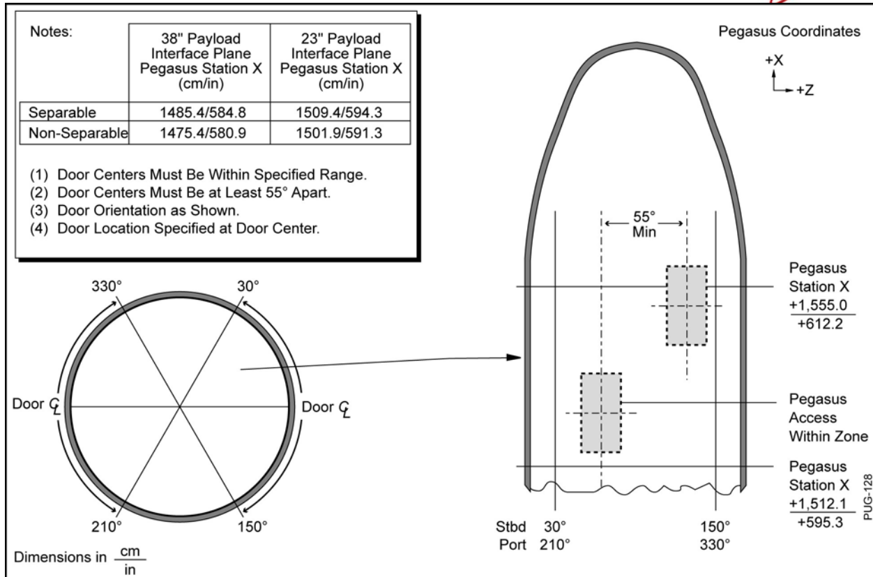
Figure 5-5. Payload Fairing Access Door Placement Zones (shown with optional second door shown)
