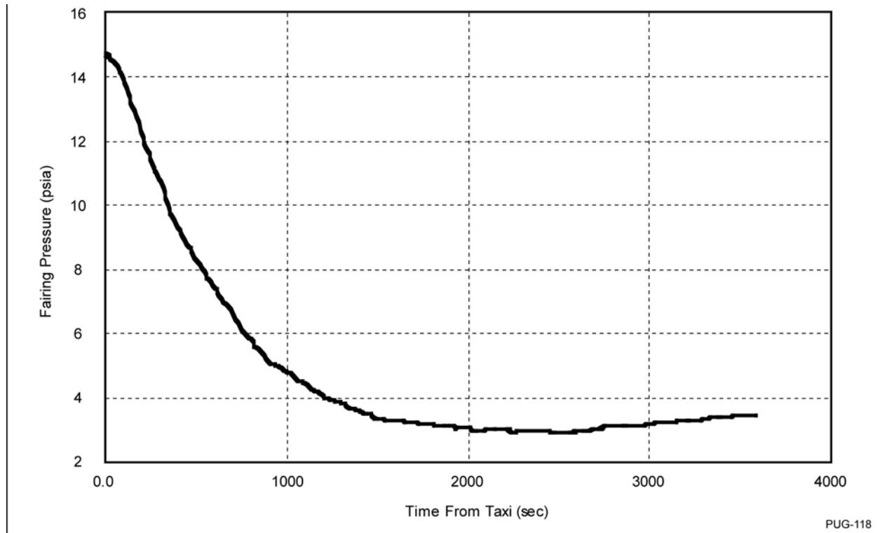
Figure 4-10. Representative Fairing Internal Pressure Profile During Captive Carry
