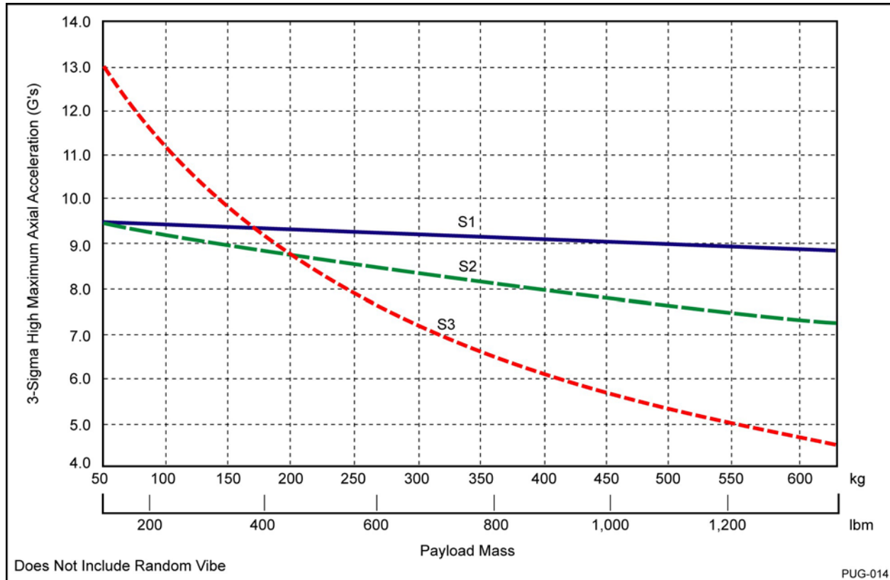
Figure 4-4. Pegasus XL Maximum Quasi Steady Acceleration as a Function of Payload Weight
