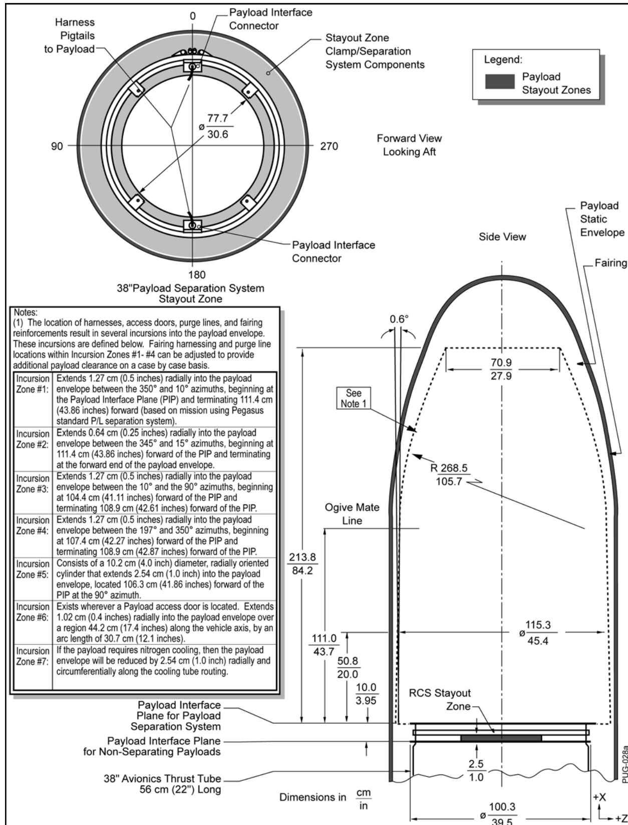
Figure 5-1. Payload Fairing Static Envelope with 97 cm (38 in.) Diameter Payload
