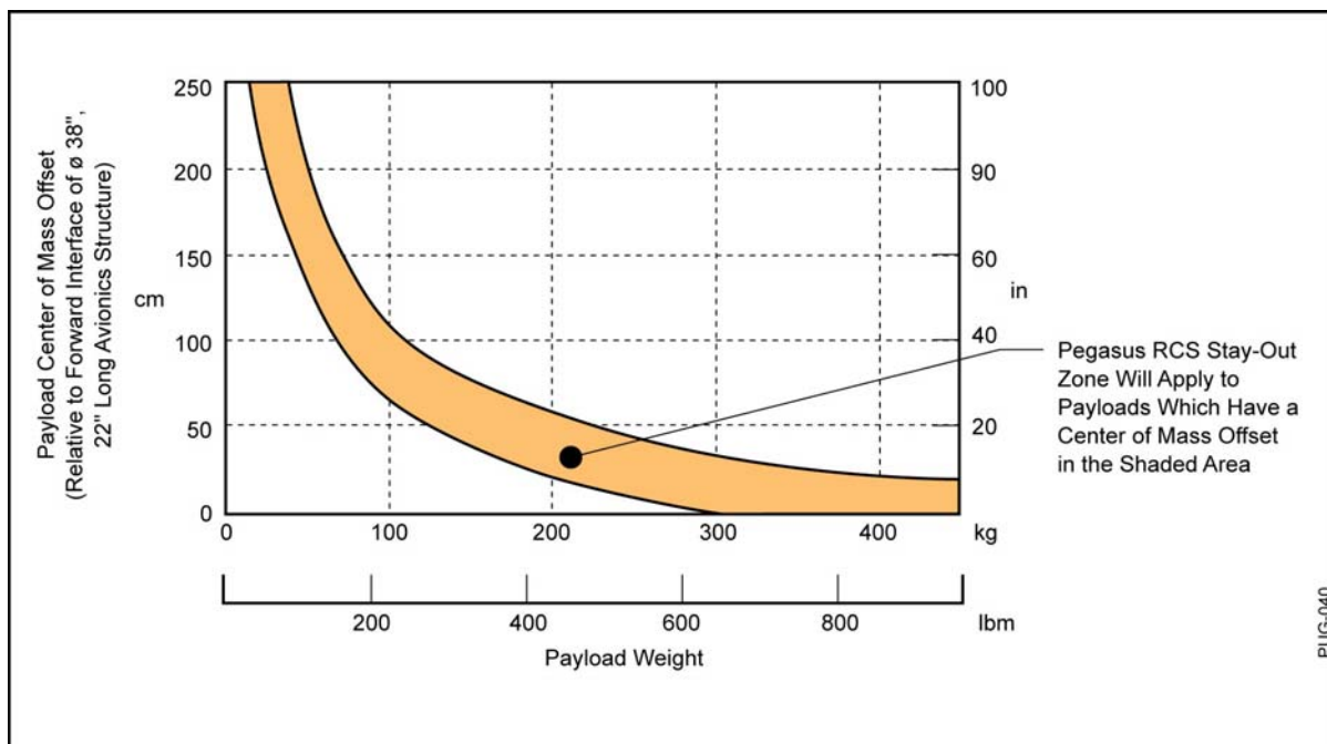
Figure 5-13. Detailed RCS Dead Band Zone
