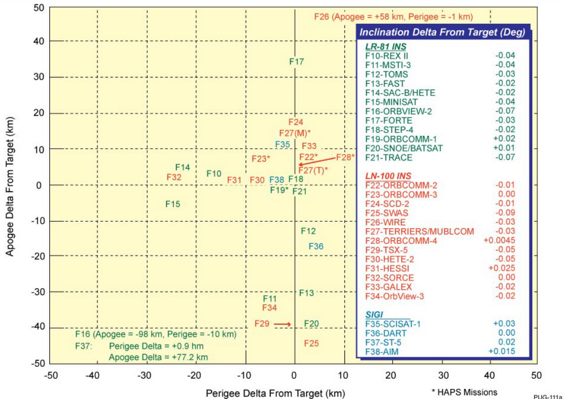
Figure 3-6. Typical and Recent Pegasus Orbital Accuracy
