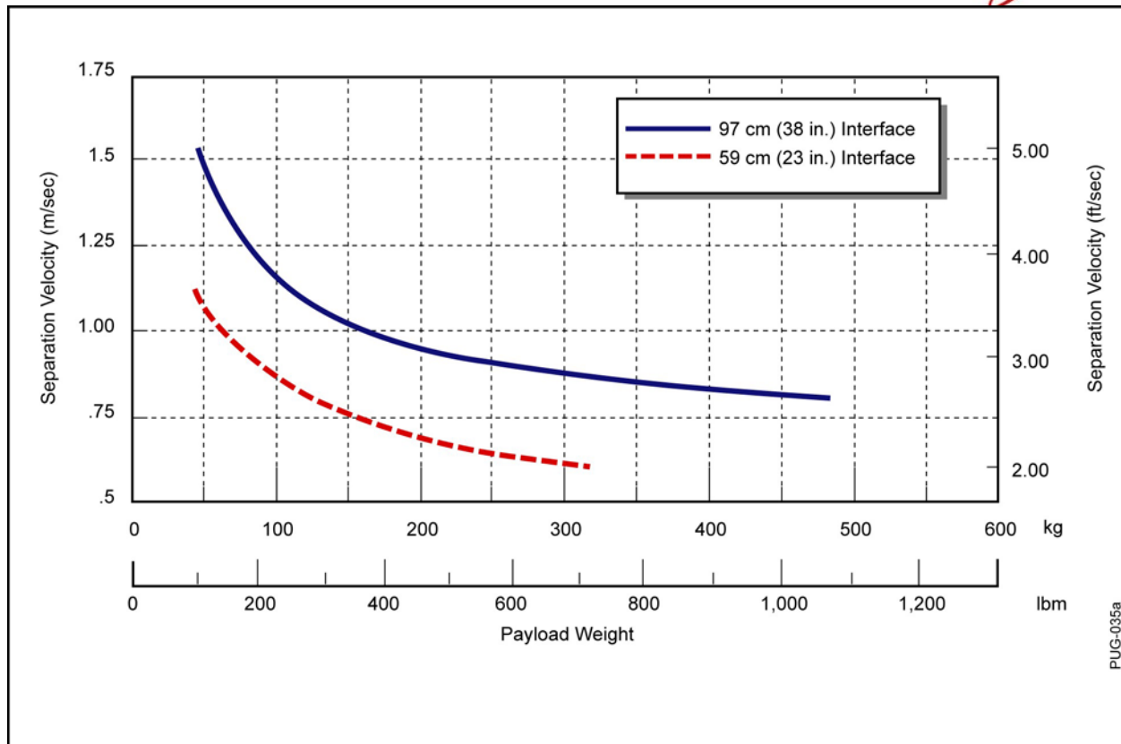
Figure 5-9. Payload Separation Velocities Using the Standard Separation System
