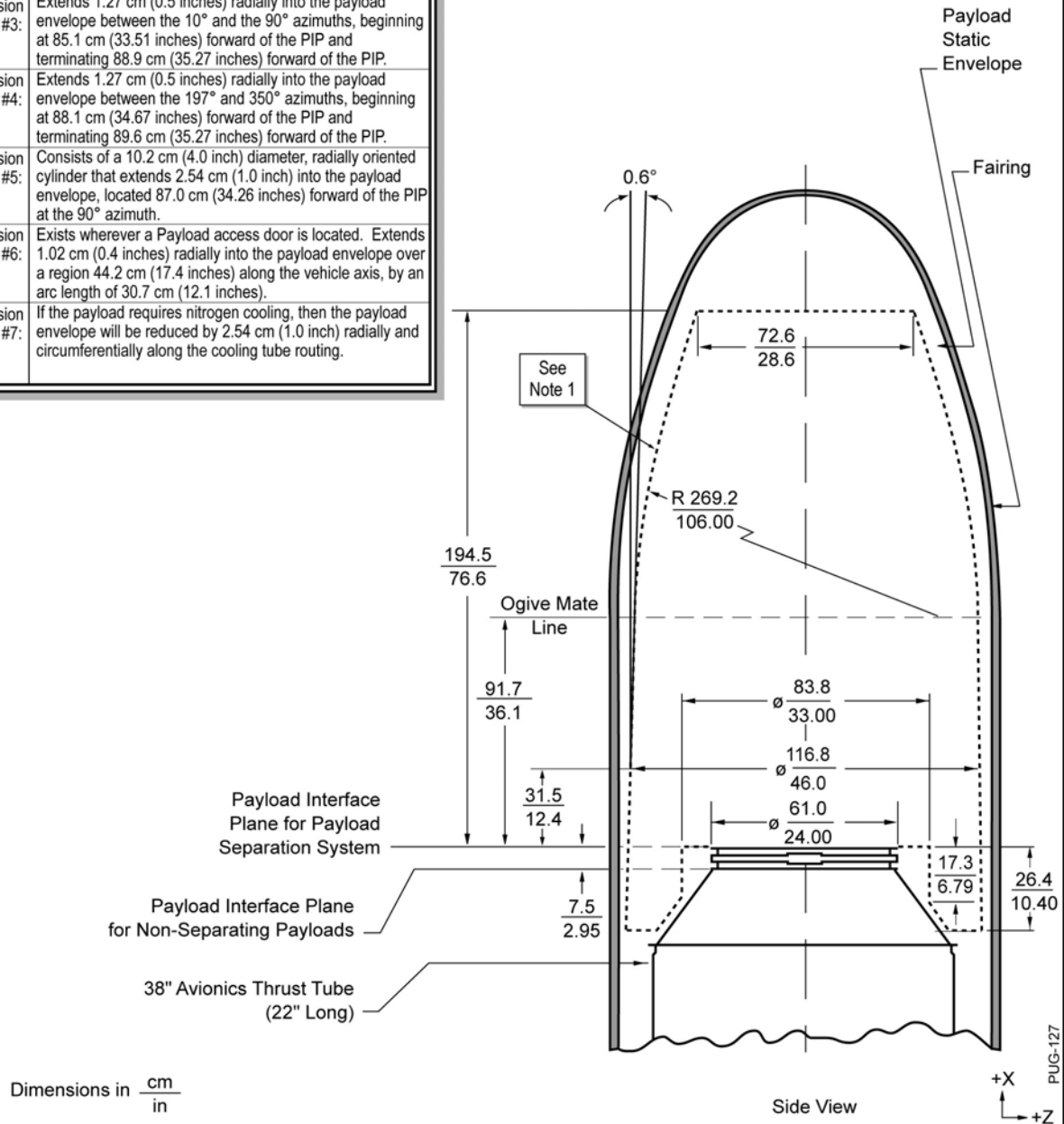
Figure 5-4. Payload Fairing Dynamic Envelope with 59 cm (23 in.) Diameter Payload
