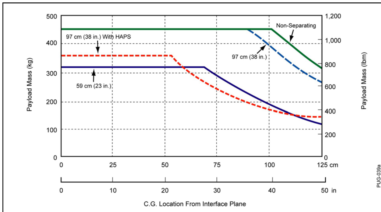
Figure 5-11. Payload Mass vs. c.g. Location on X Axis
